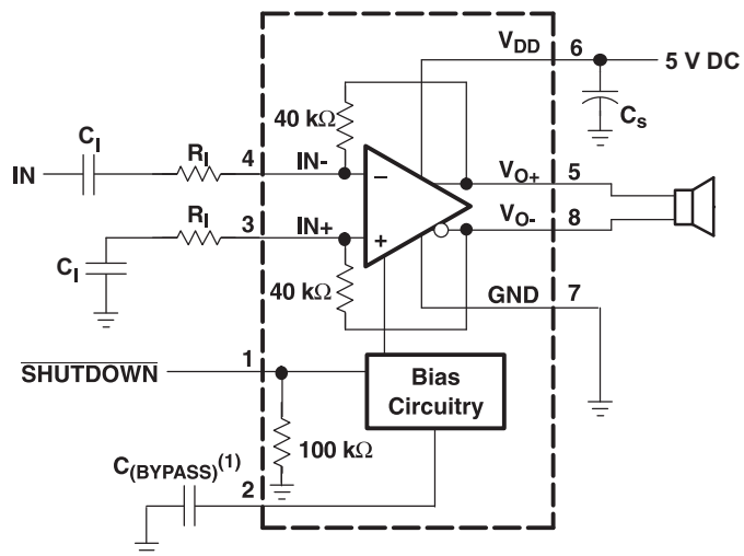
Figure 30. Single-Ended Input Application Schematic
